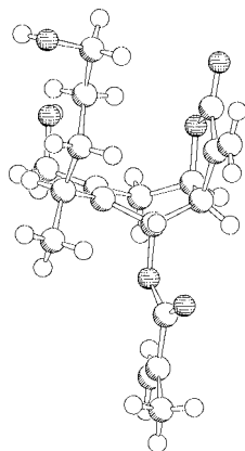
Figure 3. Crystal structure of synthetic (–)-eriolanin ( 1 ). [10,23]
