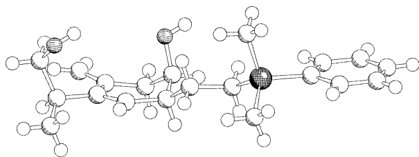
Figure 2. Crystal structure of the methylenecyclohexene 6 . [22,23]
