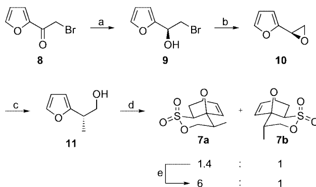
Scheme 2. Preparation of sultone 7a : a) 0.2 mol-% [Cp*RhCl(( R,R )-tsdpen)], HCO 2 H, Et 3 N, EtOAc, 0 °C, >99% ee ; b) K 2 CO 3 , MeCN, room temp.; c) MeCu(CN)Li, Et 2 O, –78 °C to room temp., 50% (3 steps), >98.5% ee ; d) \beta -chloroethanesulfonic acid chloride, Et 3 N, CH 2 Cl 2 , room temp.; e) cat. BHT, EtOAc, 120 °C, microwaves, 80% 7a (2 steps).
