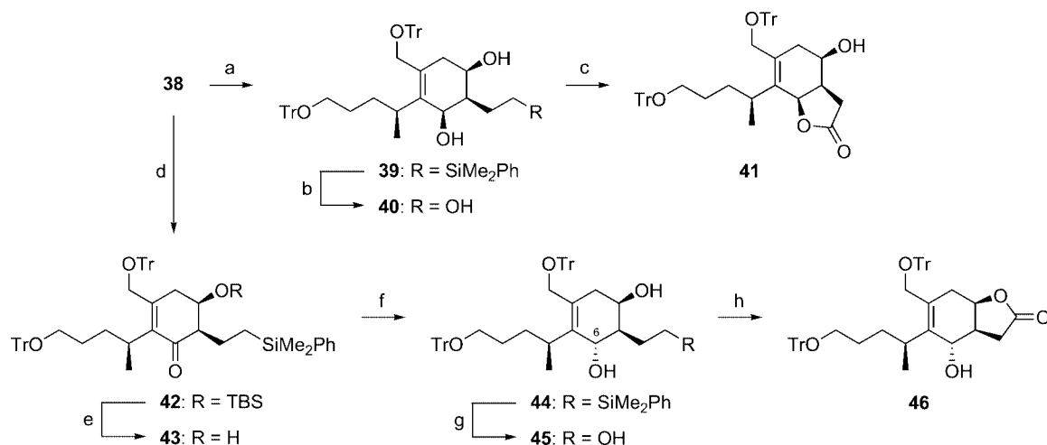
Scheme 7. Synthesis of lactone 41 and completion of the bicyclic framework 46 : a) TBAF, HOAc, THF, room temp., 97%; b) (i) TBAF, MS (4 Å), THF, 100 °C, sealed tube, (ii) KF, H 2 O 2 , NaHCO 3 , THF, MeOH, 100 °C, sealed tube, 88%; c) cat. TEMPO, NCS, TBACl, K 2 CO 3 , NaHCO 3 , CH 2 Cl 2 , H 2 O, room temp., 84%; d) Dess–Martin periodinane, pyridine, CH 2 Cl 2 , room temp., 99%; e) TBAF, HOAc, THF, room temp., 96%; f) Red-Al, CH 2 Cl 2 , PhMe, −20 °C to room temp., 90%; g) (i) TBAF, MS (4 Å), THF, reflux, (ii) KF, H 2 O 2 , NaHCO 3 , THF, MeOH, reflux, 99%; h) cat. TEMPO, bis(acetoxy)iodobenzene, CH 2 Cl 2 , room temp., 75%.
