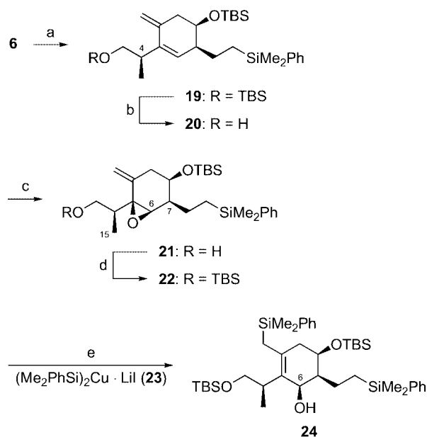
Scheme 4. 1,4-Difunctionalization of the 1,3-diene subunit, part I: a) TBSCl, imidazole, DMAP, DMF, room temp., 99%; b) TBAF, THF, 0^{\circ}\text{C} , 81% 20 + 17% 6 ; c) m CPBA, \text{NaHCO}_3 , \text{CH}_2\text{Cl}_2 , \text{H}_2\text{O} , 0^{\circ}\text{C} ; d) TBSCl, imidazole, DMAP, \text{CH}_2\text{Cl}_2 , 0^{\circ}\text{C} ; e) 23 , THF, \text{Et}_2\text{O} , -20^{\circ}\text{C} to 0^{\circ}\text{C} , 50% (3 steps).
