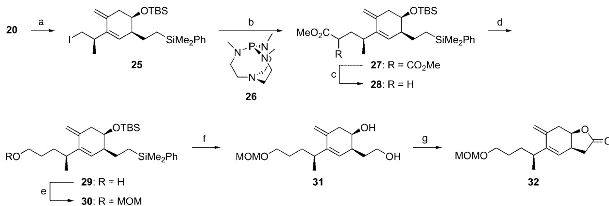
Scheme 5. Side-chain elongation and synthesis of the lactone 32 : a) I 2 , Ph 3 P, imidazole, THF, MeCN, –20 °C to room temp., 84%; b) 26 , dimethyl malonate, MeCN, room temp., 91%; c) PhSH, K 2 CO 3 , DMF, 90 °C, 89%; d) LiAlH 4 , Et 2 O, 0 °C, 100%; e) MOMCl, Et( i Pr) 2 N, CH 2 Cl 2 , 0 °C to room temp., 99%; f) (i) TBAF, MS (4 Å), THF, reflux, (ii) KF, H 2 O 2 , NaHCO 3 , THF, MeOH, reflux, 87%; g) 10 mol-% TPAP, NMO, MS (4 Å), MeCN, 15 °C to 20 °C, ultrasound, 65%.
