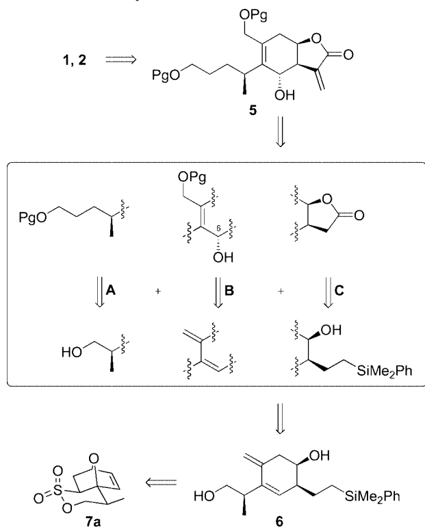
Scheme 1. Retrosynthetic analysis for eriolanin ( 1 ) and eriolangin ( 2 ).
